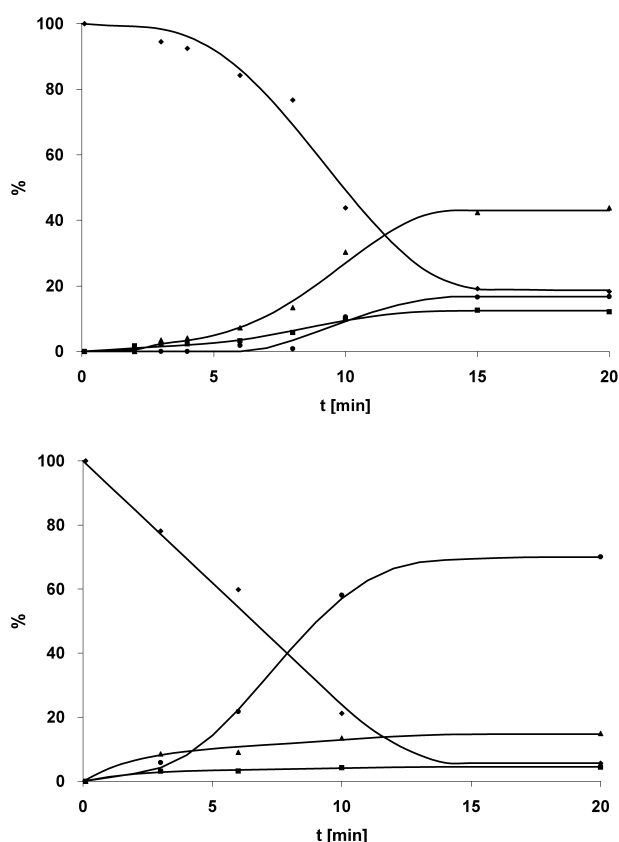
Figure 2. Yield versus time plot of the hydrosilylation of methyl undec-10-enoate 1 with triethoxysilane 2 in the solvent system cyclohexane/toluene/propylene carbonate. Conditions: 40 °C, equimolar amounts of 1 and 2 , 1 mol % \text{H}_2\text{PtCl}_6 (above: first use, below: second use). ◆: methyl undec-10-enoate 1 , ■: isomerised methyl undecenoates, ▲: methyl undecanoate, ●: hydrosilylation product 3 .
