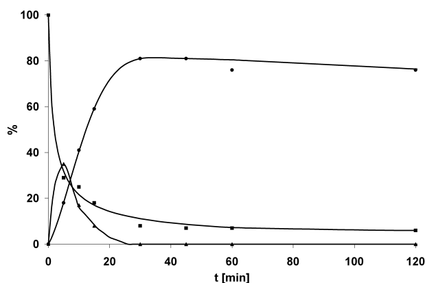
Figure 1. Yield versus time plot of the hydrosilylation of methyl linoleate 4 with chlorodimethylsilane 5 . ■: methyl linoleate 4 , ▲: conjugated methyl linoleate, ●: product 6 . 1 mol % \text{H}_2\text{PtCl}_6 , further conditions as given in Table 2.
