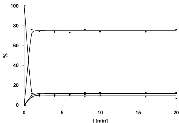
Figure 3. Yield versus time plot of the hydrosilylation of methyl undec-10-enoate 1 with triethoxysilane 2 in the solvent system cyclohexane/toluene/propylene carbonate. Conditions: 40 °C, equimolar amounts of 1 and 2 , 1 mol % Pt as Karstedt solution. ◆: methyl undec-10-enoate 1 , ■: isomerised methyl undecenoates, ▲: methyl undecanoate, ●: hydrosilylation product 3 .
